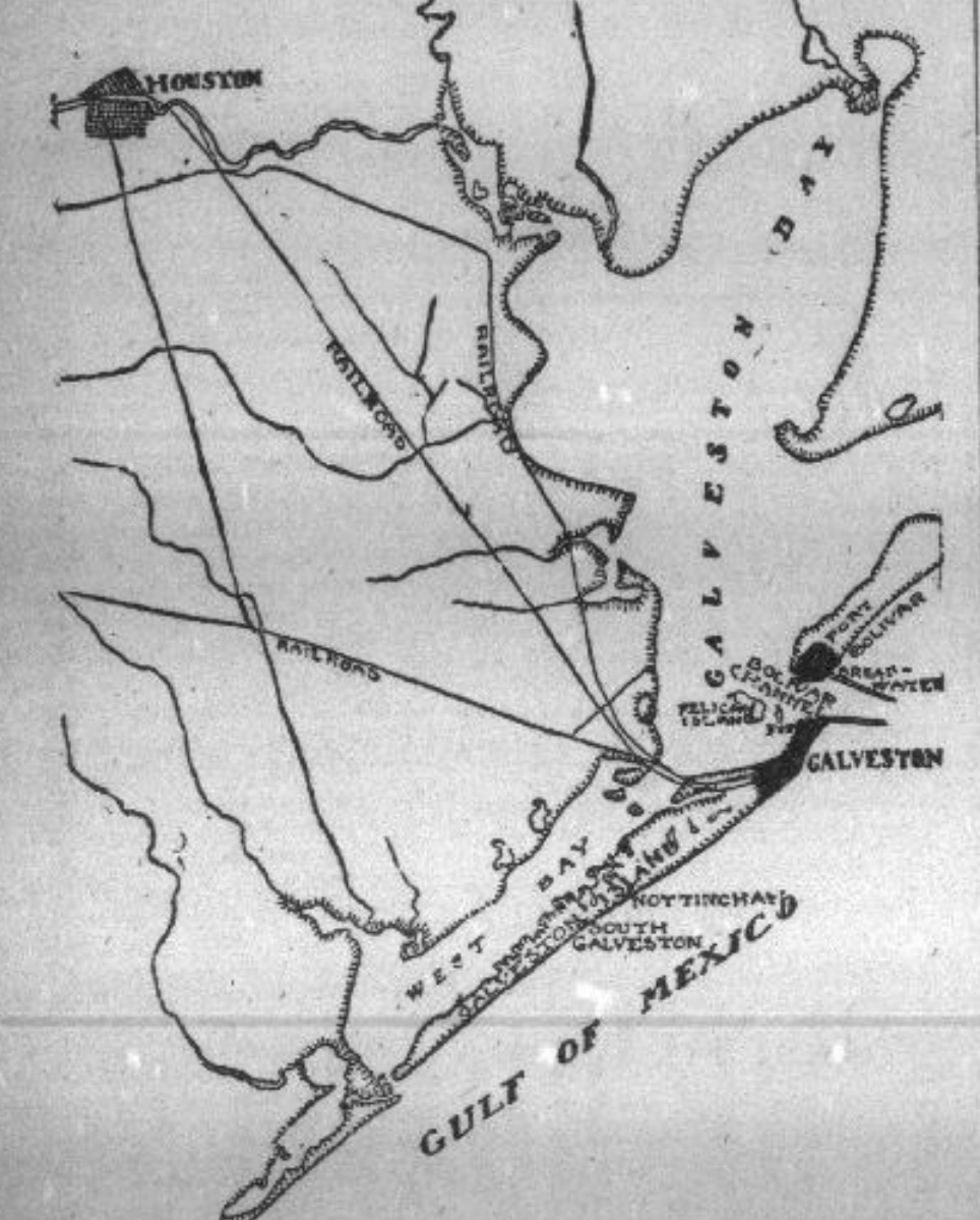
MAP SHOWING THE TRACK OF THE HURRICANE.
